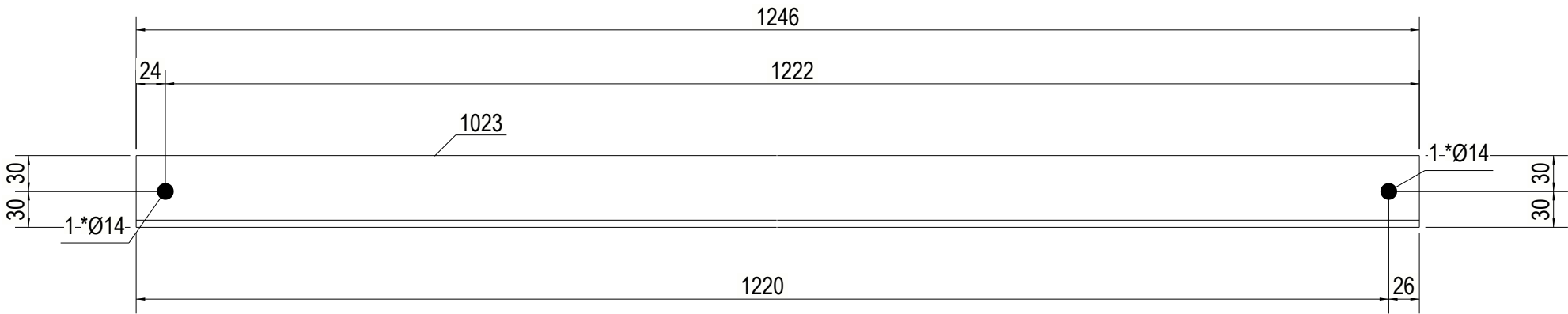
FRONT VIEW
